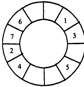
Fig. 1. n = 12 cells, k = 7 marked cells, \xi_k = 3 islands. Numbers denote the time a cell was marked.
