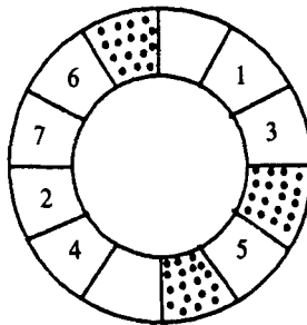
Fig. 2. Tied (shaded) and free cells.
